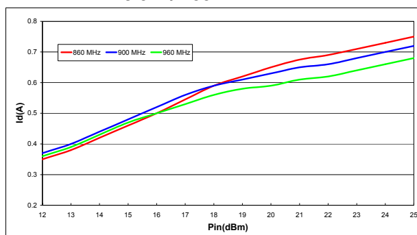
Figure 10. Id vs Pin 13.6 V / 200 mA
