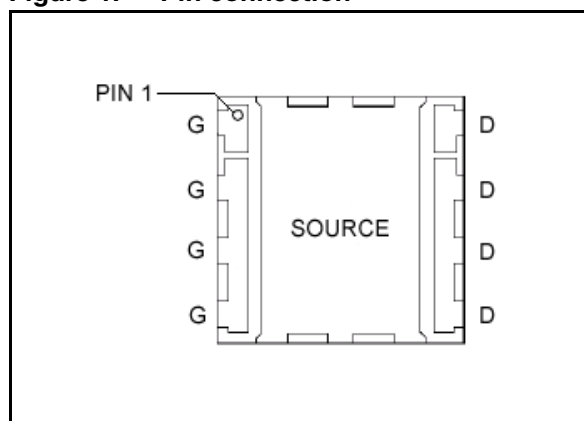
Figure 1. Pin connection
