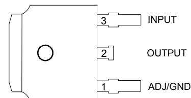
TO252-2 (3) Option 2
