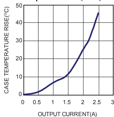
Case Temperature Rise vs. Output Current ( I_{O2}=0 )
