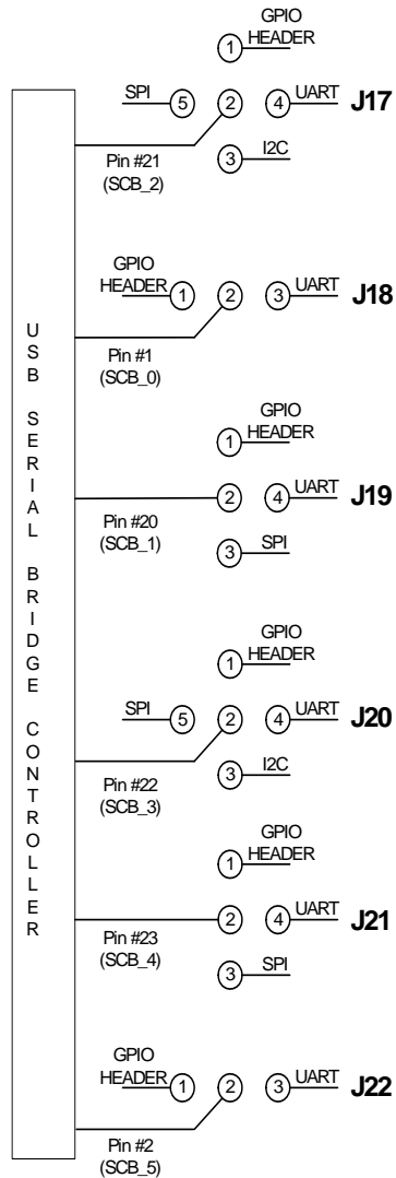
Figure 4-10. SCB Jumpers
