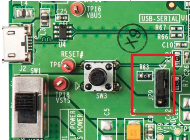
Figure 3-15. VBUS Selection Jumper
