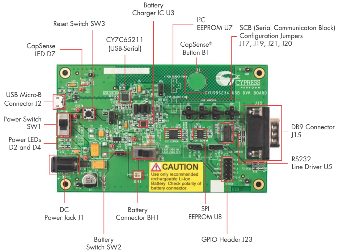
Figure 4-1. CYUSBS234 DVK Board
