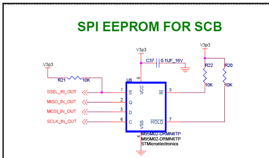
Figure 4-13. SPI Interface
