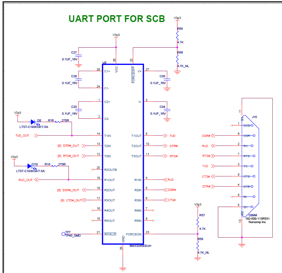
Figure 4-11. RS-232 Interface
