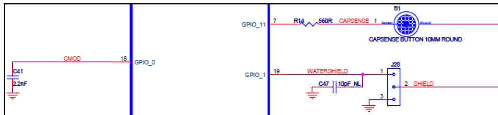
Figure A-7. CapSense Interface Circuit
