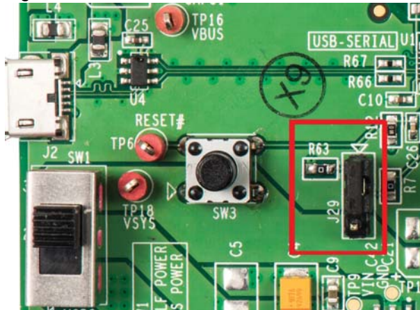
Figure 3-53. VBUS Selection
