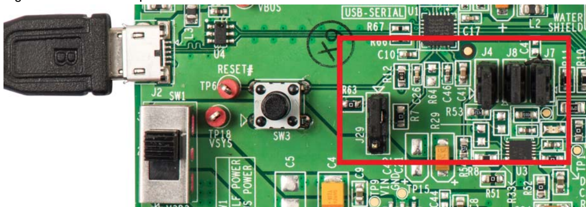
Figure 3-52. BCD Jumpers
