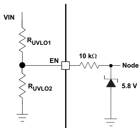
Figure 25. Internal EN Terminal Clamp
