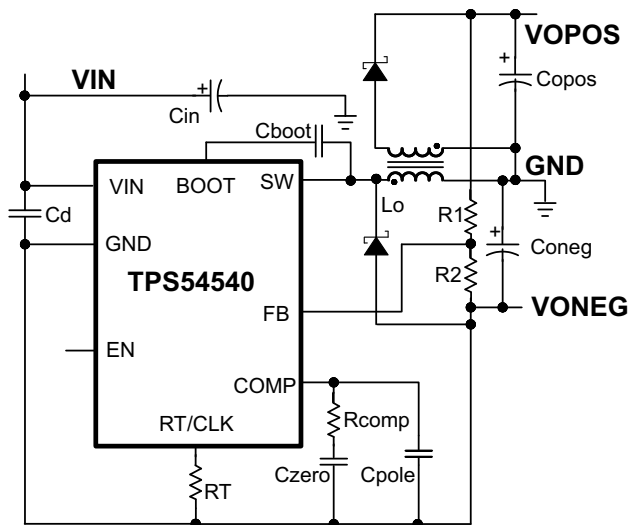
Figure 36. TPS54540 Split Rail Power Supply
