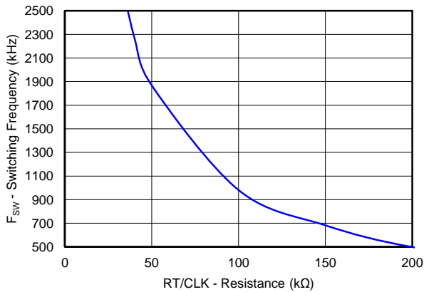
Figure 8. Switching Frequency vs RT/CLK Resistance High Frequency Range
