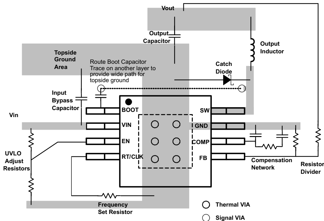
Figure 62. PCB Layout Example
