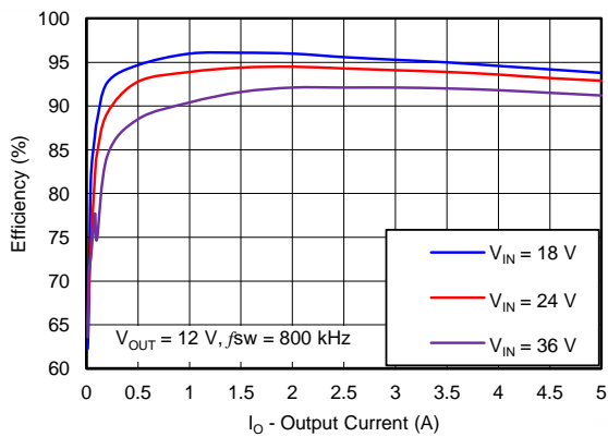
Figure 54. Efficiency vs Output Current
