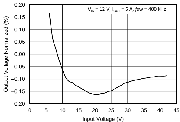
Figure 57. Regulation vs Input Voltage
