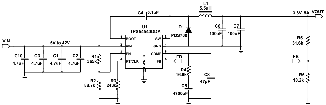
Figure 37. 3.3 V Output TPS54540 Design Example
