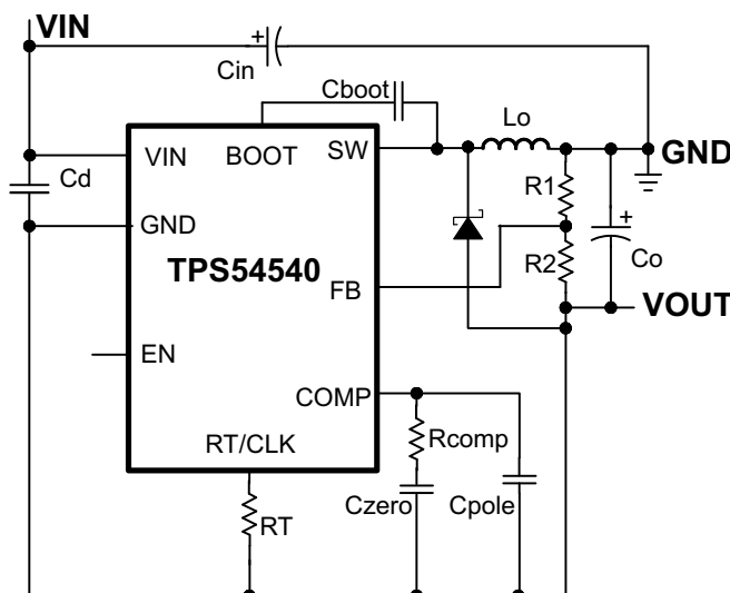
Figure 35. TPS54540 Inverting Power Supply
