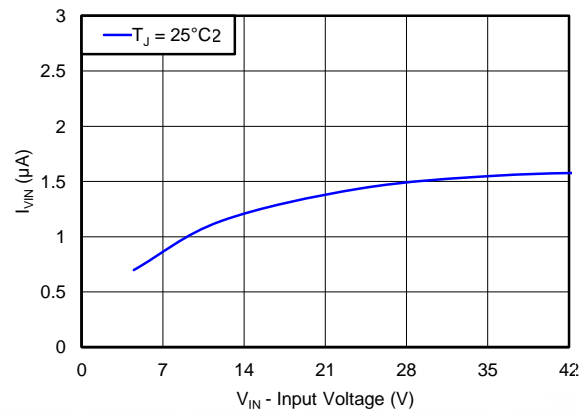
Figure 17. Shutdown Supply Current vs Input Voltage ( V_{IN} )
