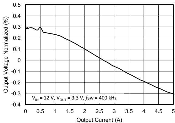
Figure 56. Regulation vs Load Current
