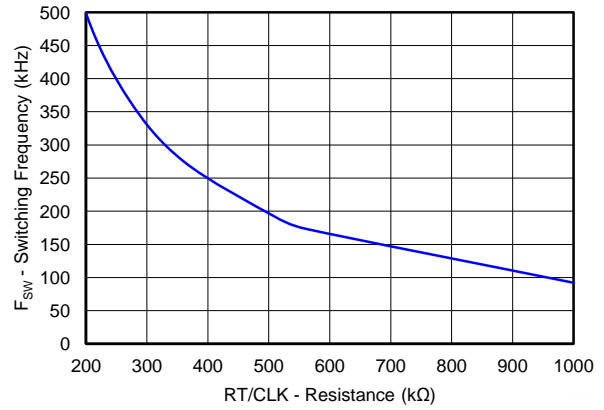
Figure 7. Switching Frequency vs RT/CLK Resistance Low Frequency Range
