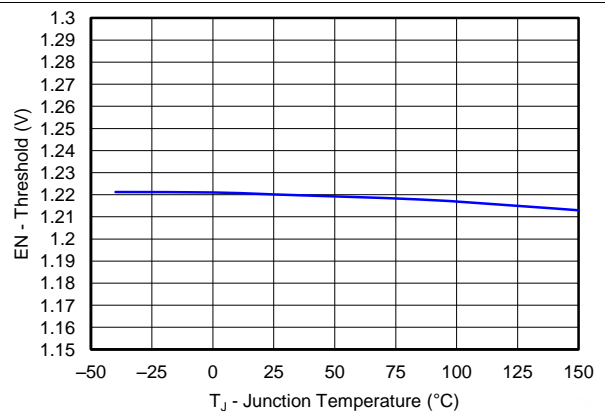
Figure 11. EN Terminal Voltage vs Junction Temperature
