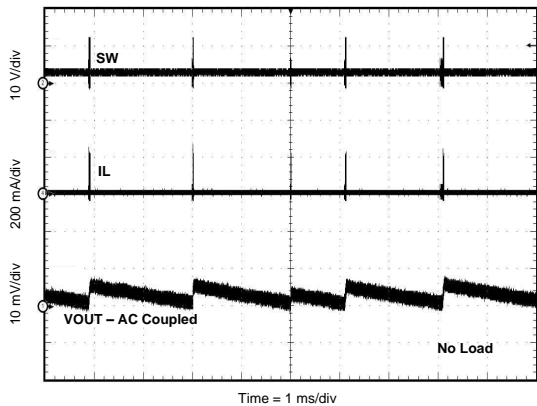
Figure 44. Output Ripple PSM
