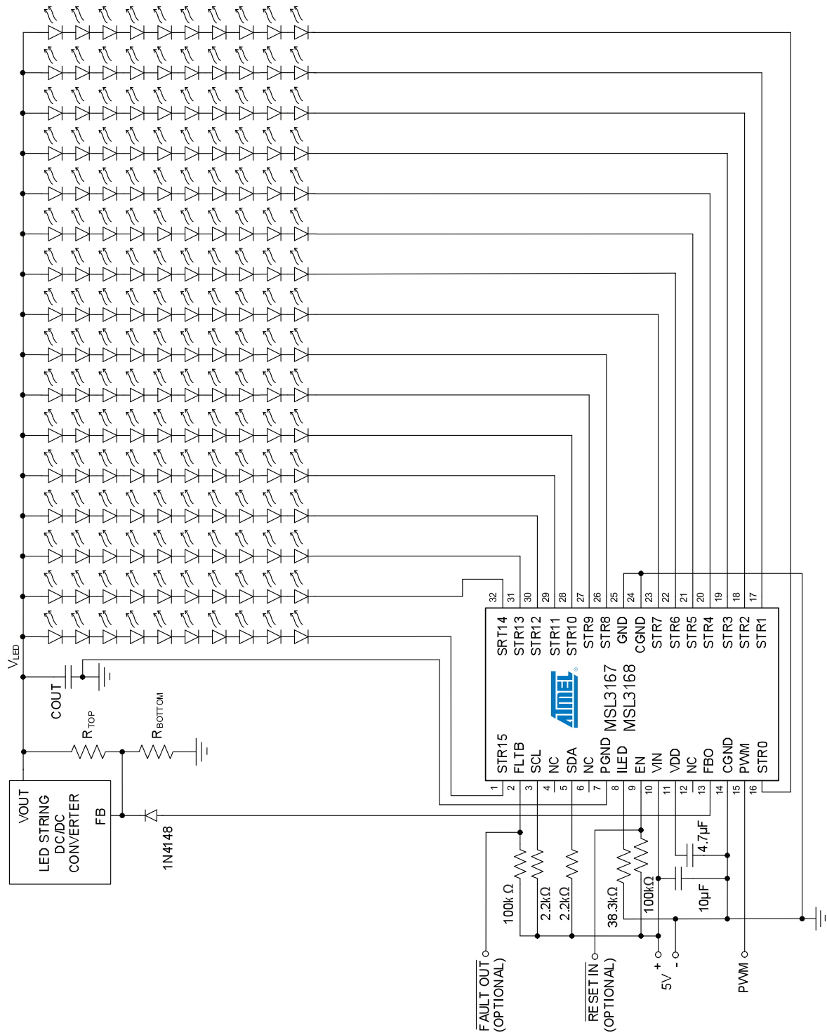
Figure 3. Atmel LED Drivers-MSL3167/8 Driving 160 White LEDs in 16 Strings at 20mA per String.
