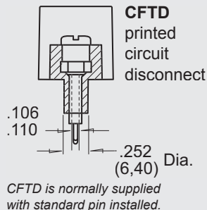
CFT turret-type solder pin
