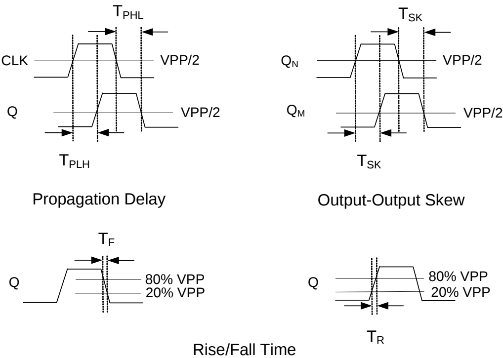
Figure 10. AC Waveforms
