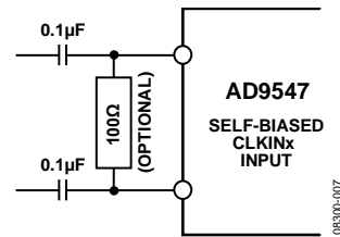
Figure 30. CLKINx Input
