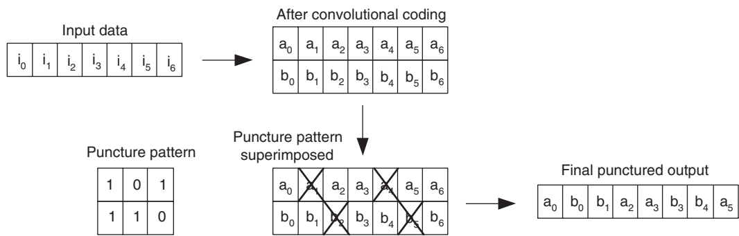
Figure 4. Puncturing Process
