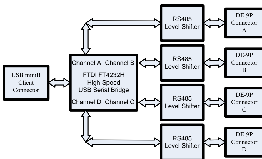
Figure 1.2 USB2-H-5004 Block Diagram
