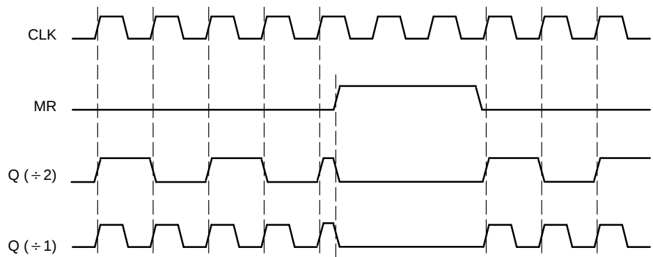
Figure 4. Master Reset (MR) Timing Diagram
