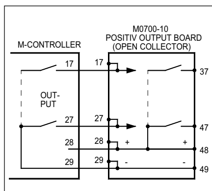
Fig. 2. M0700-10 Positive Output PC Board
