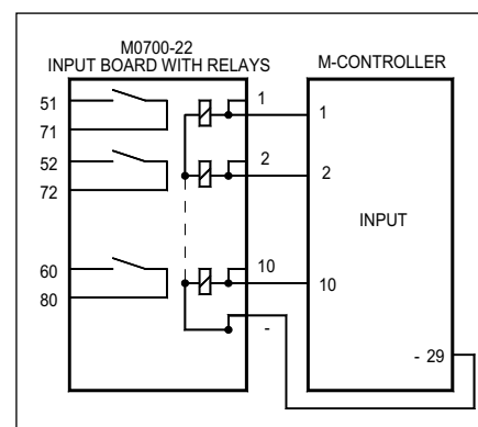
Fig. 3. M0700-22 Input Board
