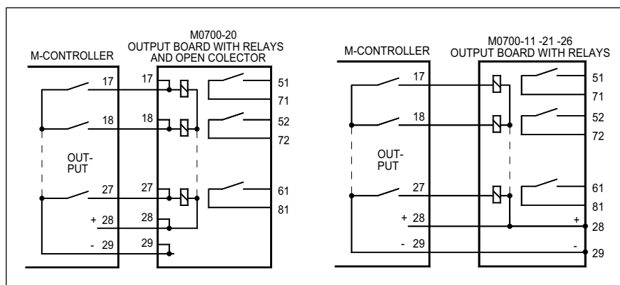
Fig. 1. M0700-20 Relay PC Board
