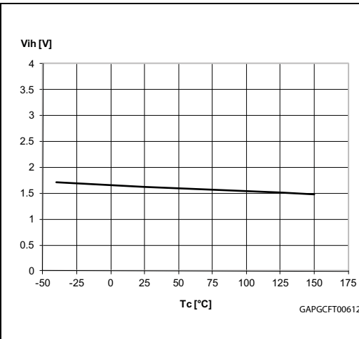
Figure 17. Input high level voltage
