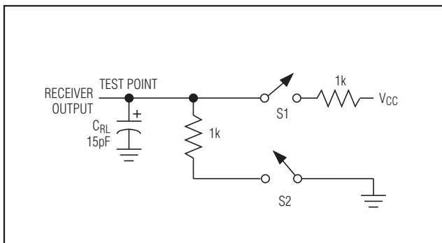
Figure 9. Receiver Timing Test Load
