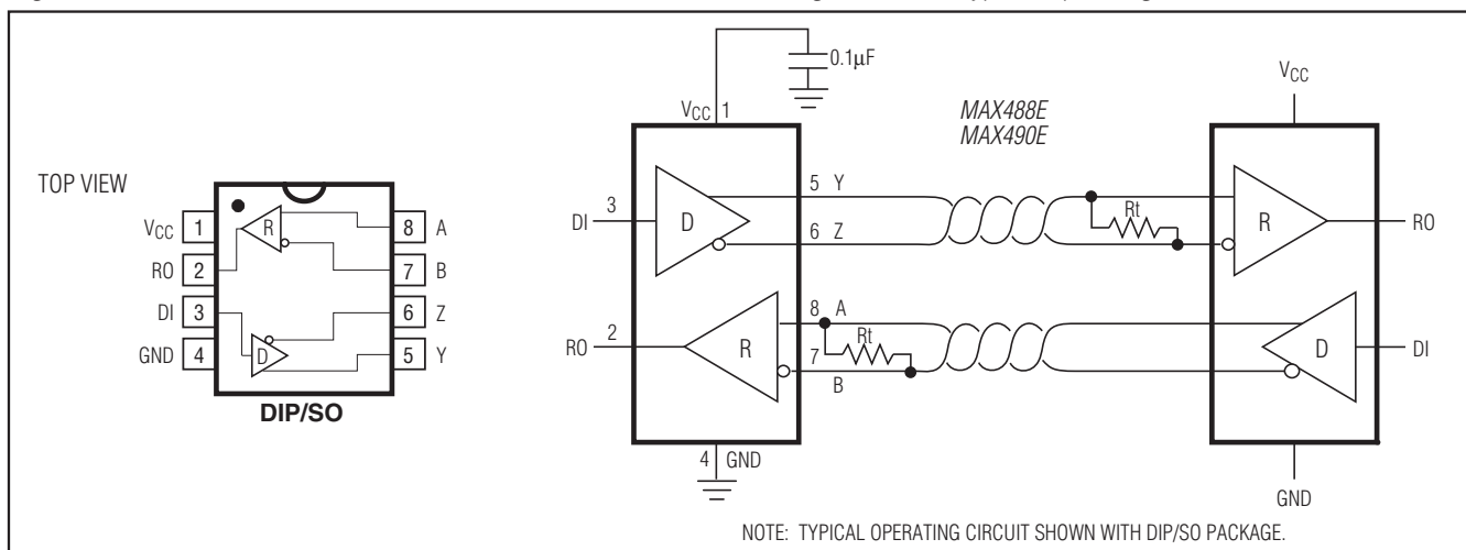
Figure 2. MAX488E/MAX490E Pin Configuration and Typical Operating Circuit
