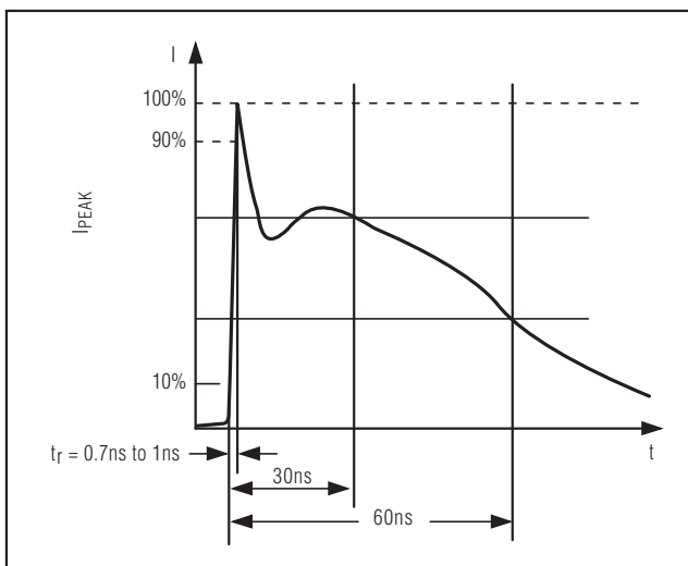
Figure 7. IEC1000-4-2 ESD Generator Current Waveform
