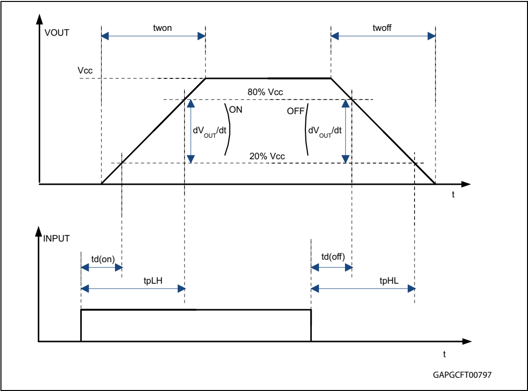
Figure 6. Switching times and Pulse skew
