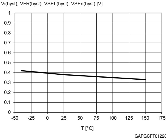
Figure 24. Undervoltage shutdown
