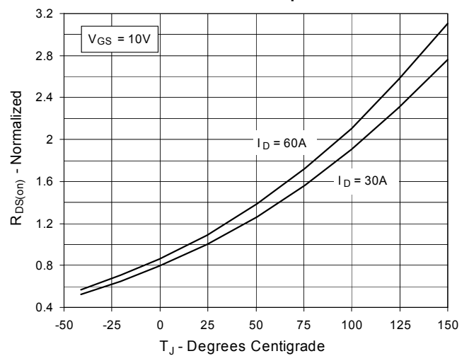
Fig. 4. R_{DS(on)} Normalized to I_D = 30\text{A} Value vs. Junction Temperature
