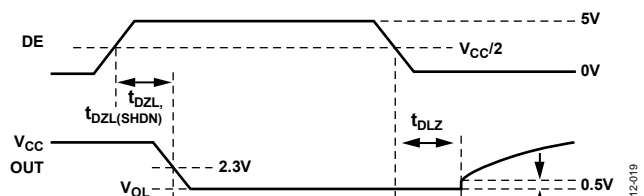
Figure 19. Driver Enable and Disable Times ( t_{DZL} , t_{DZL} , t_{DZL(SHDN)} )
