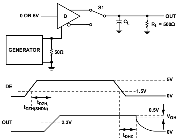
Figure 18. Driver Enable and Disable Times ( t_{DZH} , t_{DZH(SHDN)} , t_{DZL} , t_{DZL(SHDN)} , t_{DHZ} )
