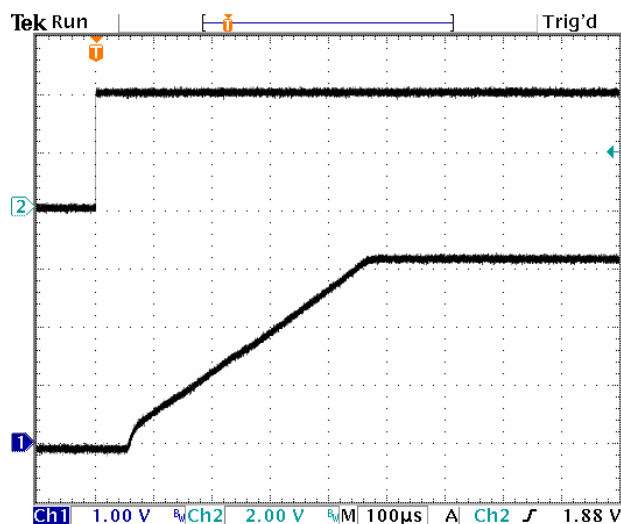
Start Up Waveform: V_{IN} = 5.0V , V_{OUT} = 3.3V ; I_{LOAD} = 500mA (VID MODE)
