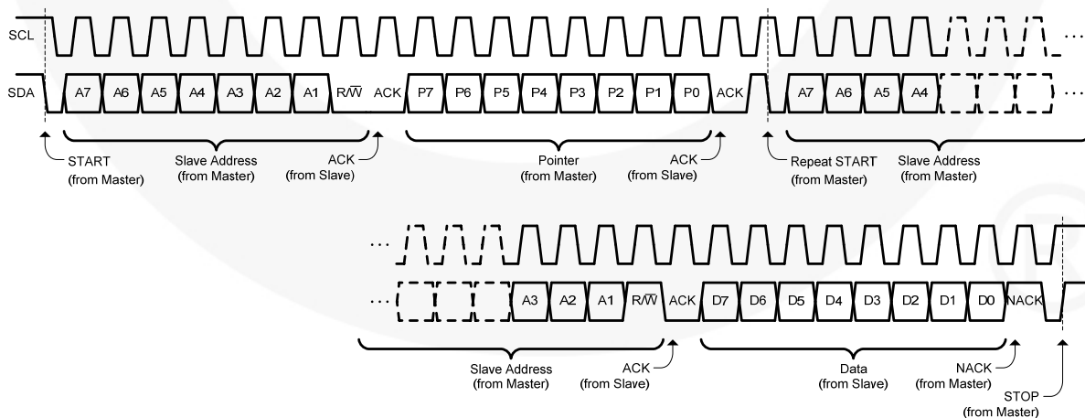
Figure 32. I²C Write Followed by Read
