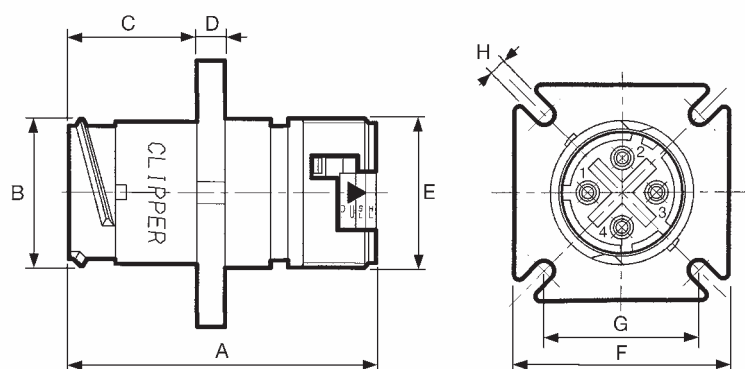
Square flange receptacle
