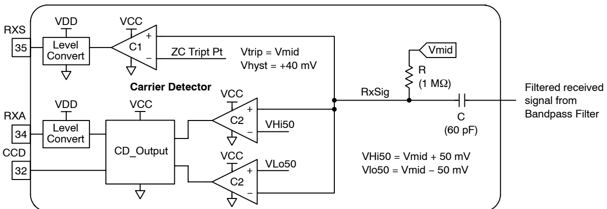
Figure 10. Receive Signal Detectors
