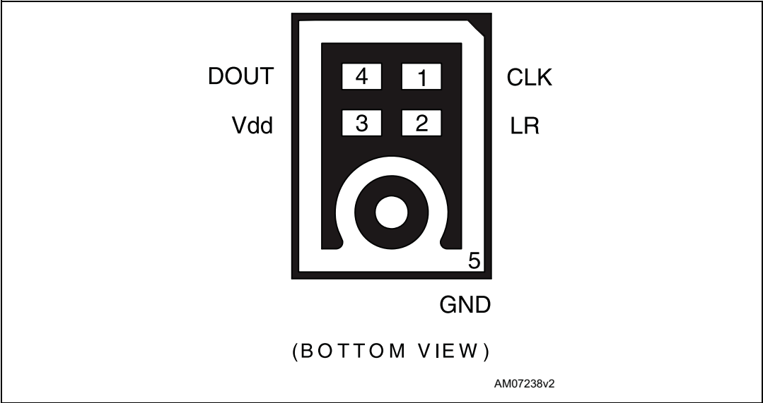
Figure 1. Pin connections
