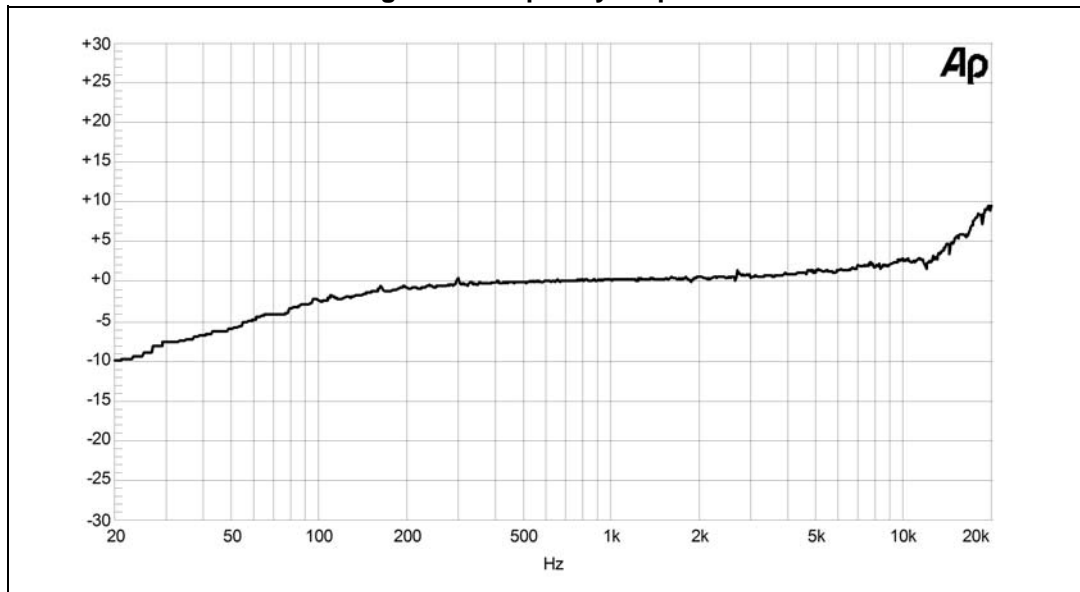
Figure 3. Frequency response
