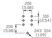
P.C.MOUNTING
