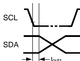
Figure 26. Data Output Timing
