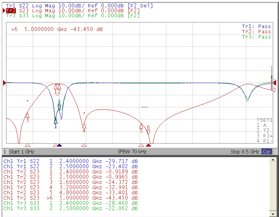
Fig. 3 Frequency Characteristics
