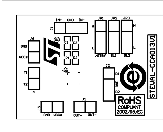
Figure 2. PCB top overlay
