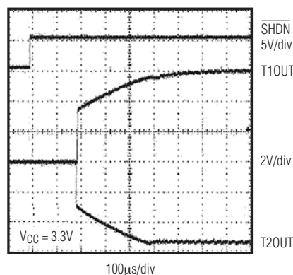
Figure 3. Transmitter Outputs when Exiting Shutdown or Powering Up
