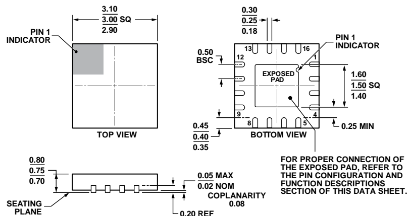
Figure 22. 16-Lead Lead Frame Chip Scale Package [LFCSP_WQ]
