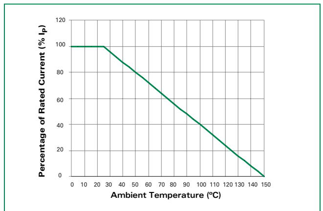
Current Derating Curve
