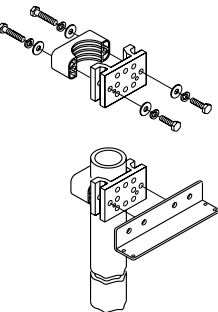
LCMK-4
