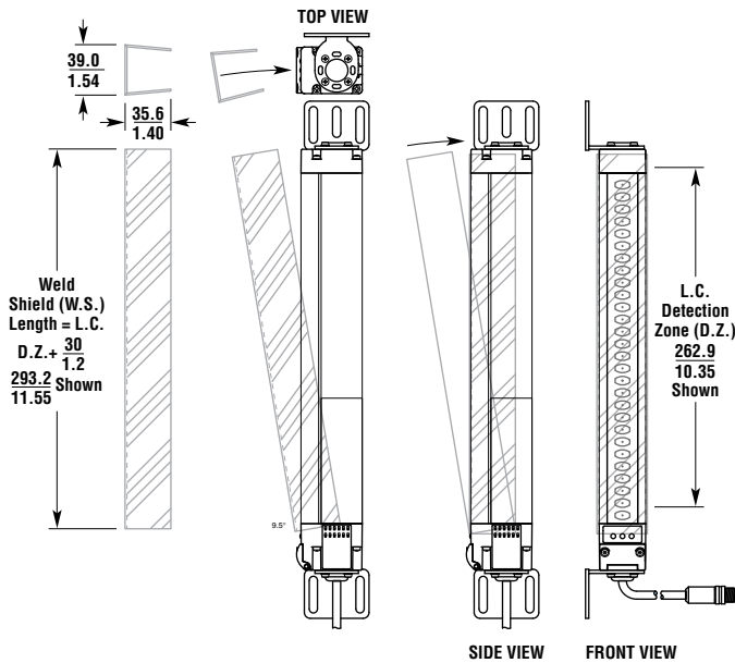
MS4800 Light Curtain (L.C.)
