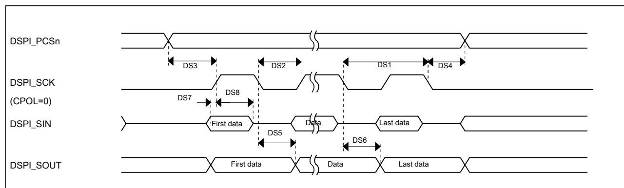
Figure 23. DSPI classic SPI timing — master mode
