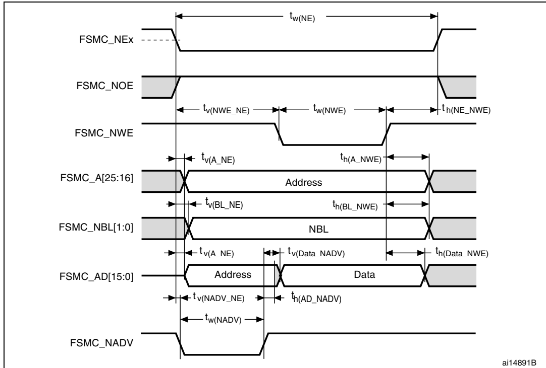
Figure 57. Asynchronous multiplexed PSRAM/NOR write waveforms
