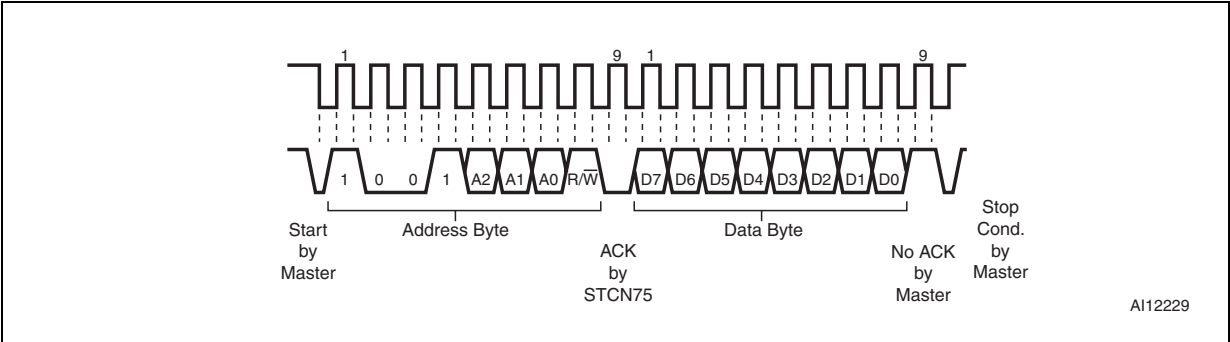
Figure 10. Typical 1-byte READ from the configuration register with preset pointer
