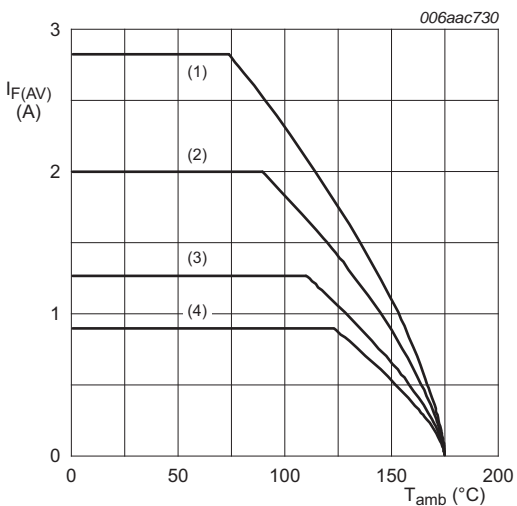
FR4 PCB, mounting pad for cathode 1\text{ cm}^2 T_j = 175\text{ }^{\circ}\text{C} (1) \delta = 1.0 (2) \delta = 0.9 (3) \delta = 0.8 (4) \delta = 0.5
