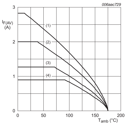
FR4 PCB, standard footprint T_j = 175\text{ }^{\circ}\text{C} (1) \delta = 1.0 (DC) (2) \delta = 0.5 ; f = 20\text{ kHz} (3) \delta = 0.2 ; f = 20\text{ kHz} (4) \delta = 0.1 ; f = 20\text{ kHz}
