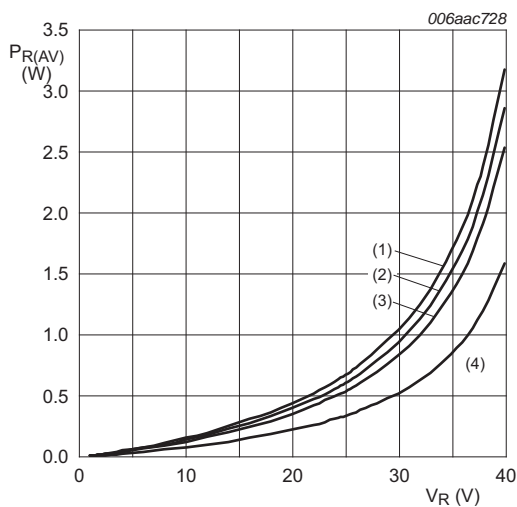
T_j = 150\text{ }^{\circ}\text{C} (1) \delta = 1.0 (2) \delta = 0.9 (3) \delta = 0.8 (4) \delta = 0.5
