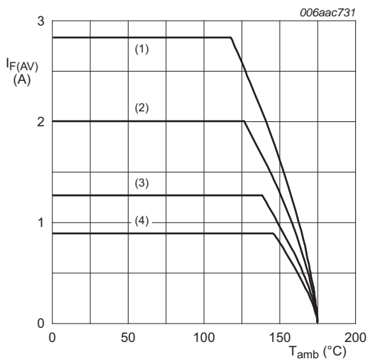
Ceramic PCB, \text{Al}_2\text{O}_3 , standard footprint T_j = 175\text{ }^{\circ}\text{C} (1) \delta = 1.0 (DC) (2) \delta = 0.5 ; f = 20\text{ kHz} (3) \delta = 0.2 ; f = 20\text{ kHz} (4) \delta = 0.1 ; f = 20\text{ kHz}
