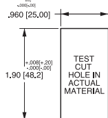
VMS MOUNTING PANEL HOLE
