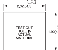
MOUNTING PANEL OPENING (2) UNITS
