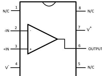
SOIC-8 (LMH6645) Package D08A Top View
