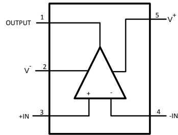
SOT-23-5 (LMH6645) Package DBV05A Top View
