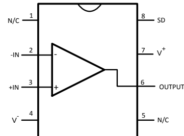
SOIC-8 (LMH6647) Package D08A Top View
