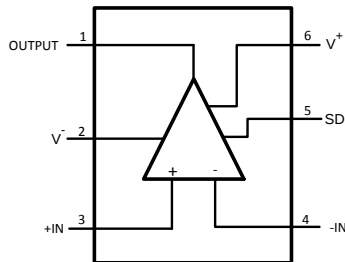
SOT-23-6 (LMH6647) Package DBV06A Top View
