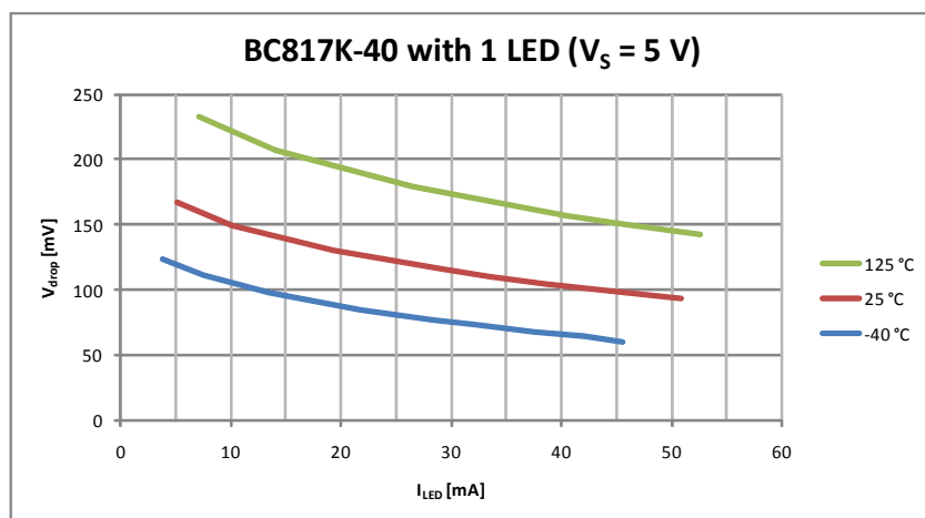
Figure 11 Drop Voltage vs. LED current in 1 LED Application with BC817K-40
