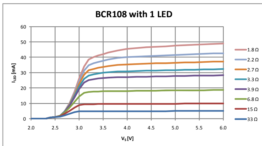
Figure 6 LED Current vs. Supply Voltage in 1 LED Application with BCR108
