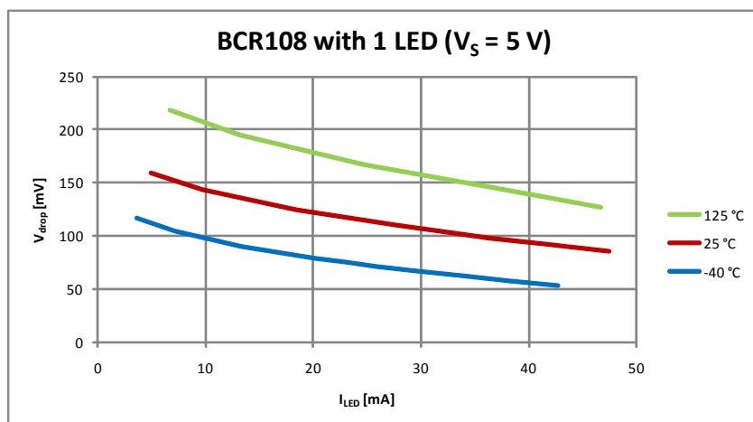
Figure 8 Drop Voltage vs. LED current in 1 LED Application with BCR108
