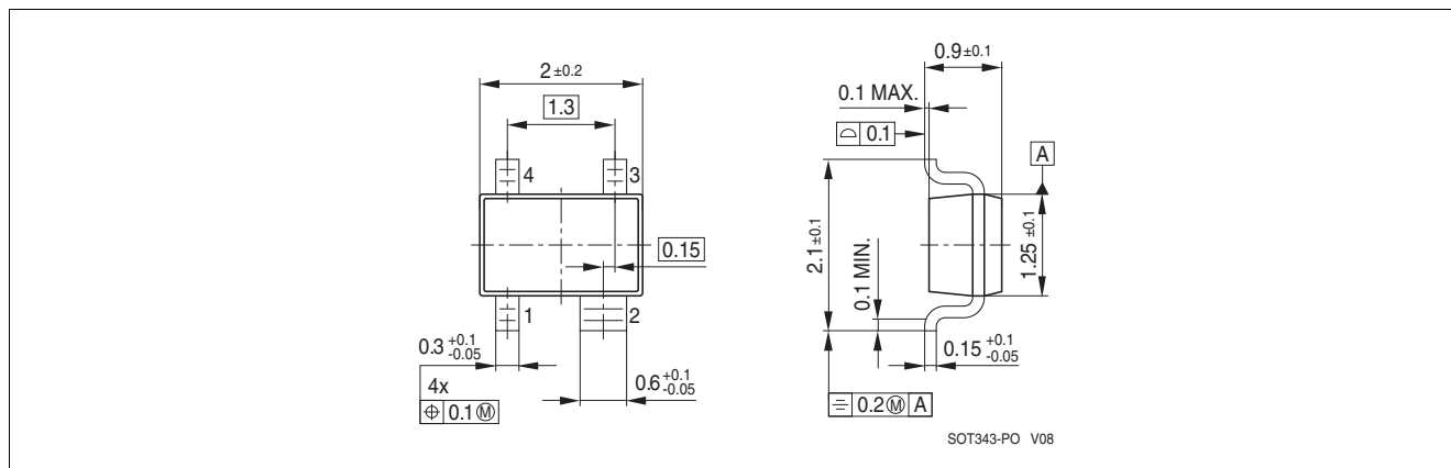
Figure 15 Package outline
