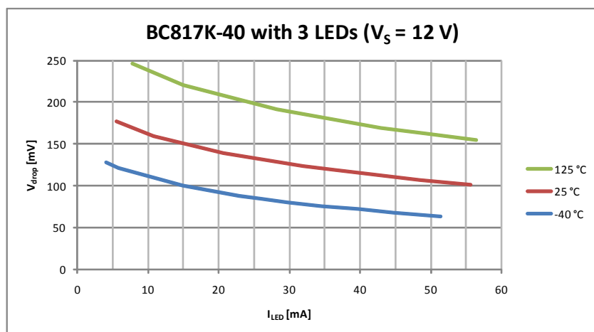
Figure 14 Drop Voltage vs. LED current in 3 LED Application with BC817K-40
