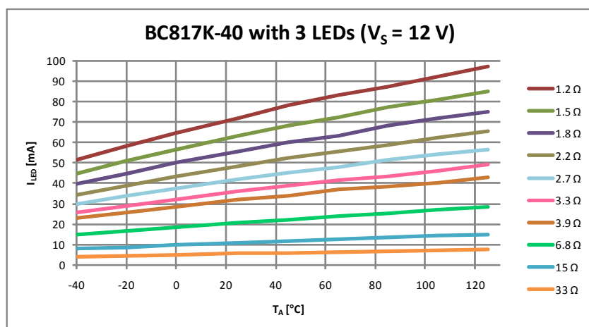
Figure 13 LED Current vs. Ambient Temperature in 3 LED Application with BC817K-40
