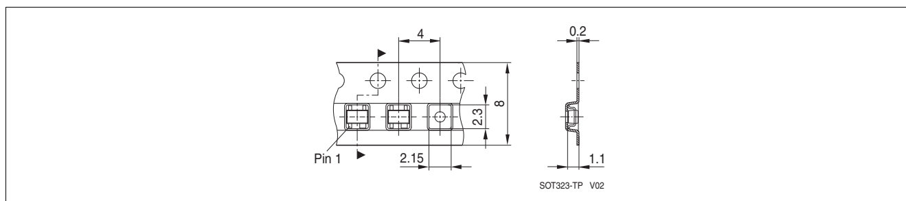
Figure 17 Tape Loading
