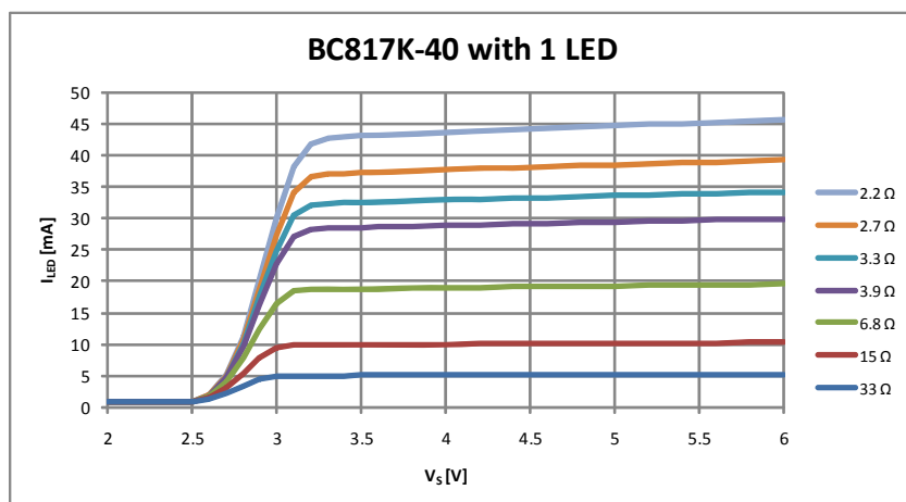
Figure 9 LED Current vs. Supply Voltage in 1 LED Application with BC817K-40
