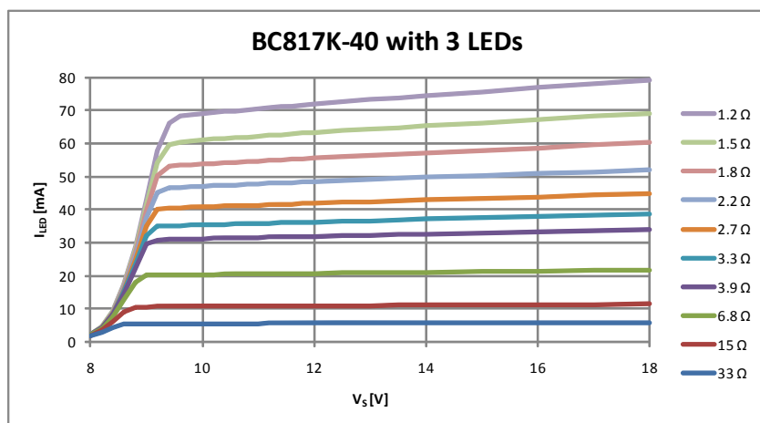
Figure 12 LED Current vs. Supply Voltage in 3 LED Application with BC817K-40
