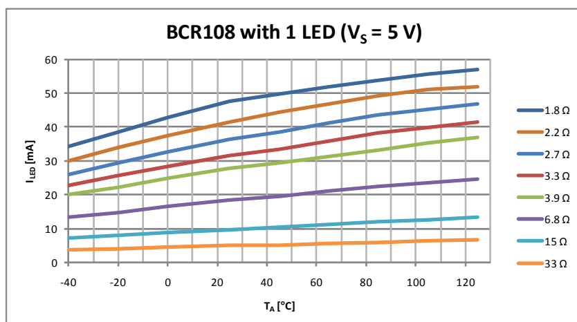
Figure 7 LED Current vs. Ambient Temperature in 1 LED Application with BCR108
