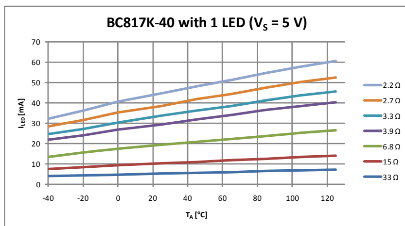
Figure 10 LED Current vs. Ambient Temperature in 1 LED Application with BC817K-40
