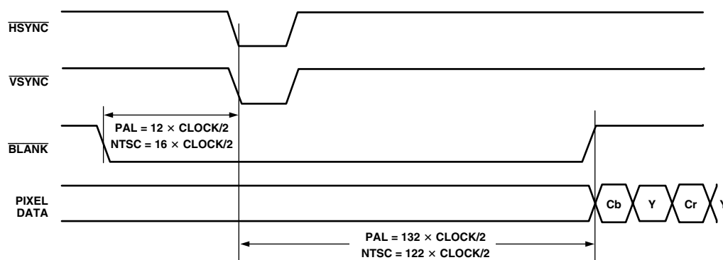
Figure 103. SD Timing Mode 2 Even to Odd Field Transition, Master/Slave
