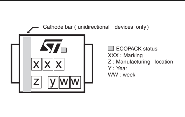
Figure 11. Marking layout
