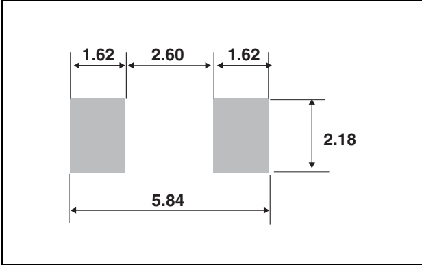
Figure 10. Footprint dimensions (millimeter)
