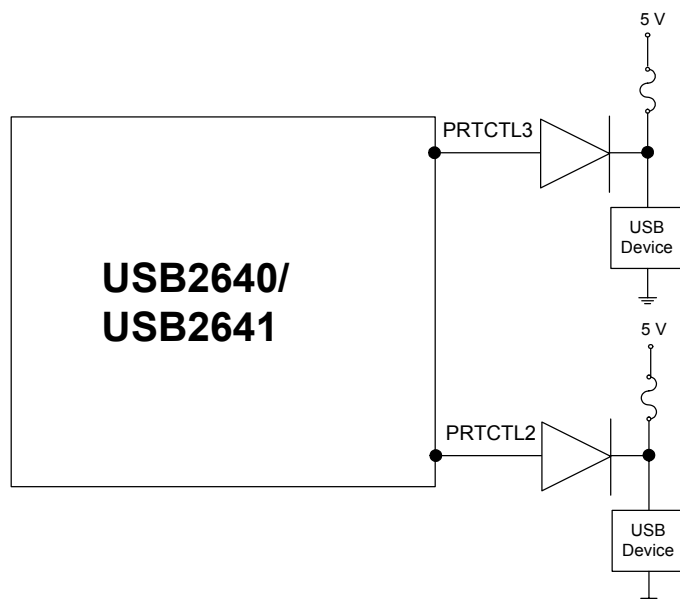
Figure 6.2 Port Power Control with Single Poly Fuse and Multiple Loads
