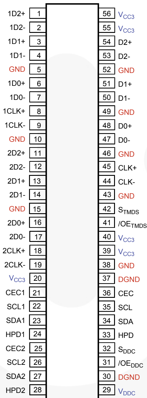
Figure 3. Pin Assignments
