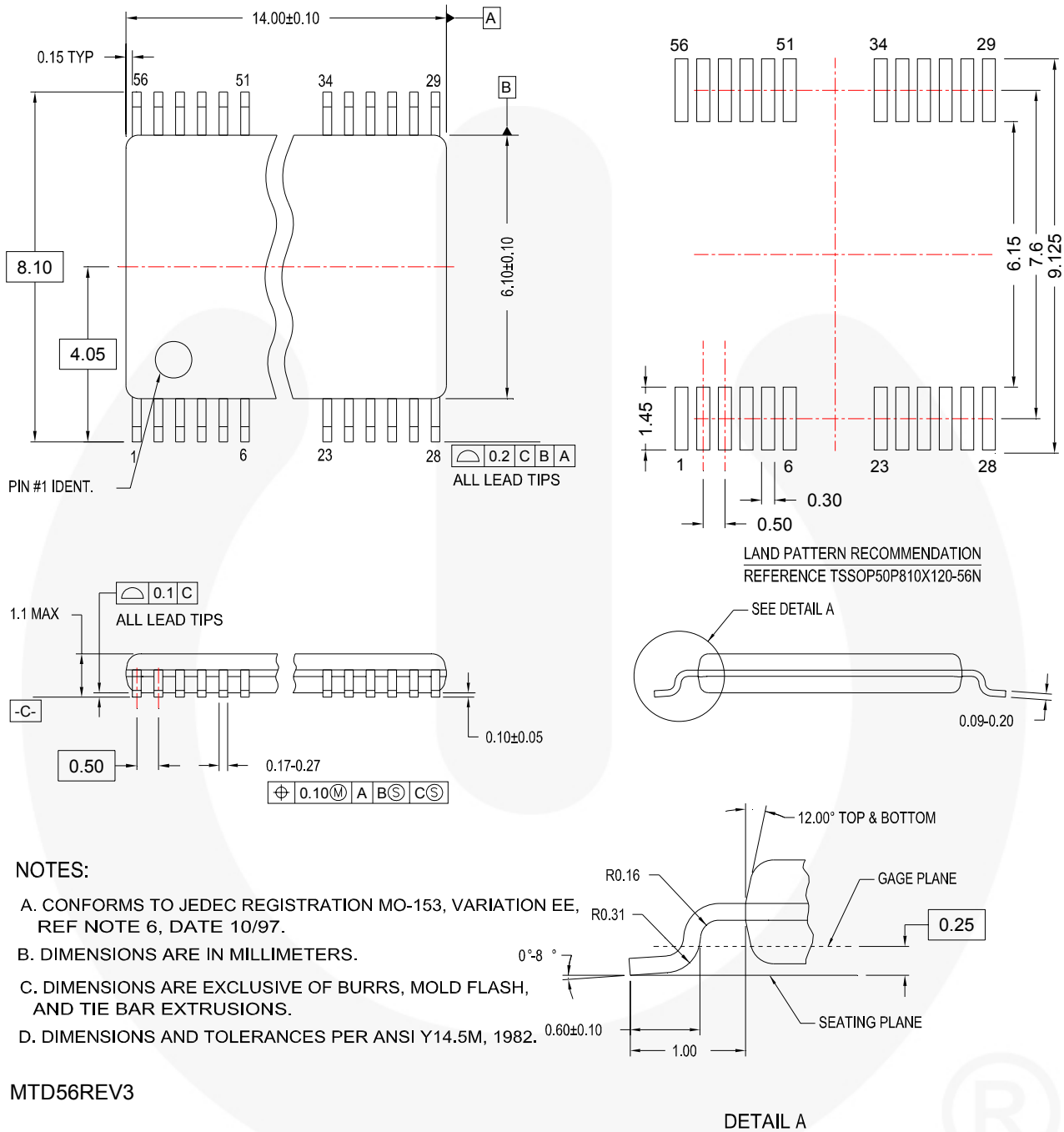
Figure 16. 56-Pin Thin-Shrink Small Outline Package (TSSOP)
