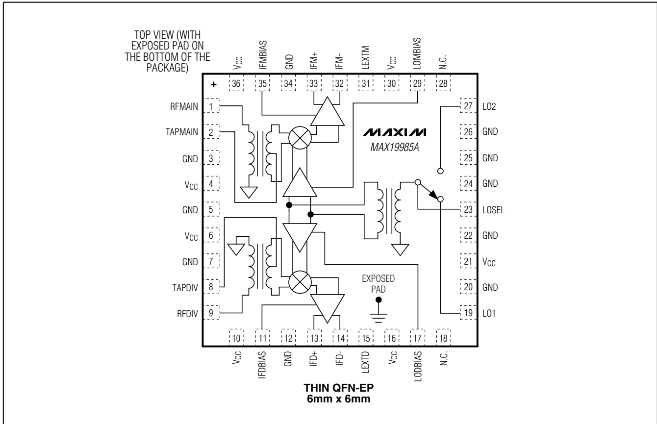
Pin Configuration/Functional Diagram
