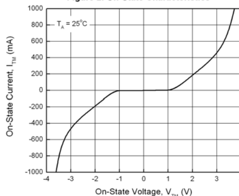
Figure 2. On-State Characteristics
