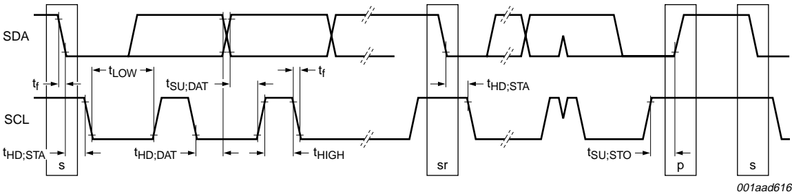
Fig 11. Timing diagram
