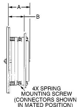
DLD Assembly Dimensions
