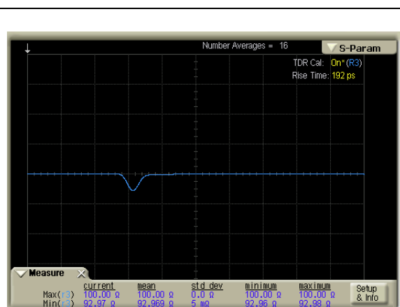
Figure 15. TDR measurement
