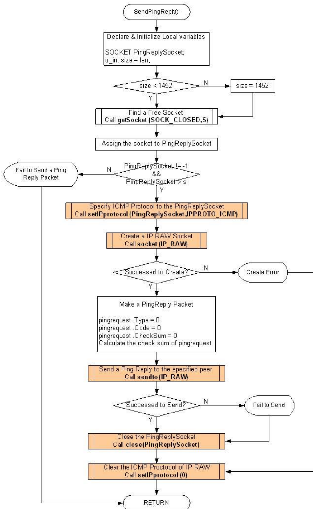
<Fig 3.13: SendPingReply()>
