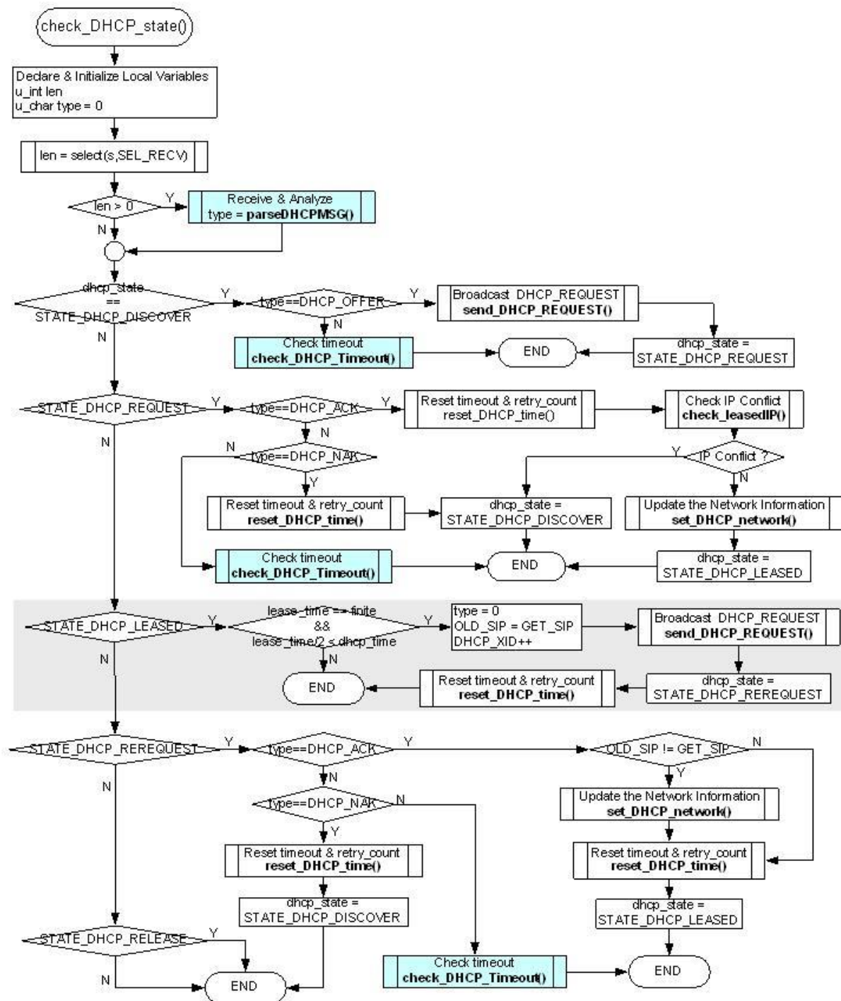
<Fig 3.31: check_DHCP_state()>
