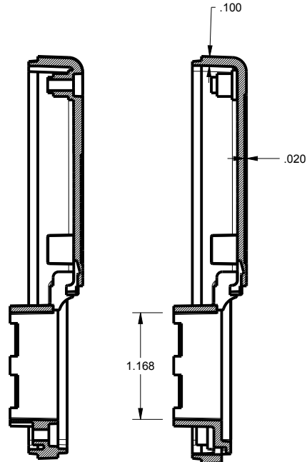
SECTION C-C
