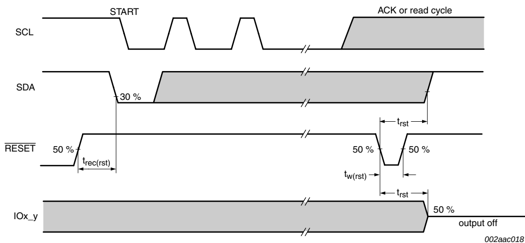
Fig 39. Reset timing
